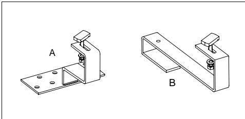
Abb.3 Dachanker
